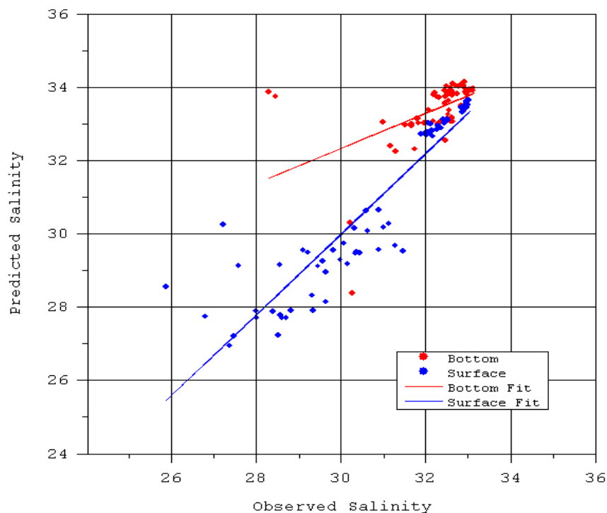
Figure 5-3. Comparison of EFDC predicted and observed salinity at 20 stations for four sampling times during the December 2004 to March 2005 period using NOAA Port wind fields
