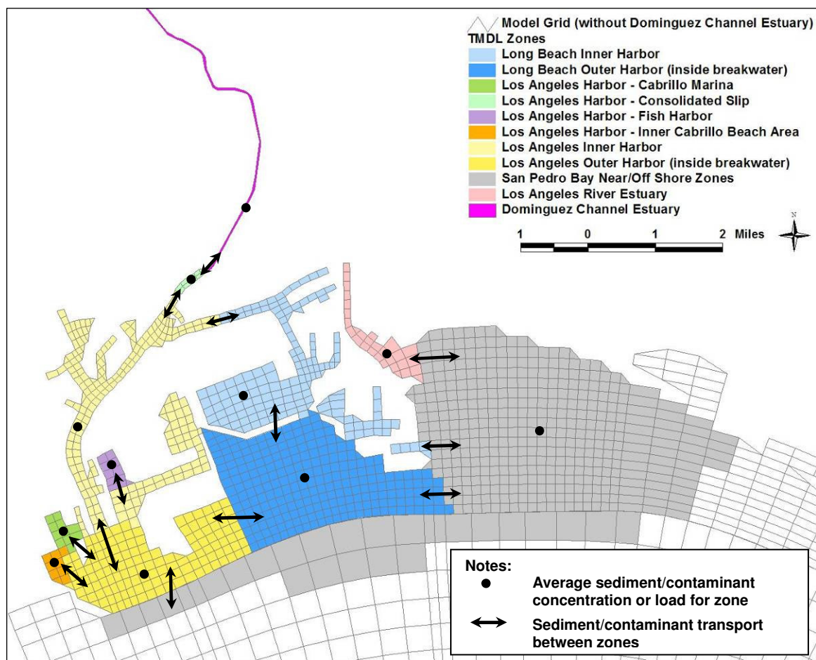
Figure 5-4. TMDL (EFDC) model zones
