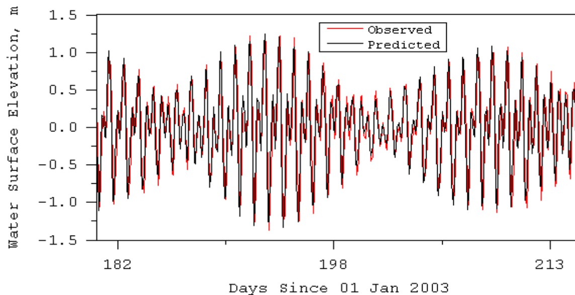
Figure 5-2. Tidal water surface elevation comparison at NOAA tide gauge in Los Angeles Harbor
