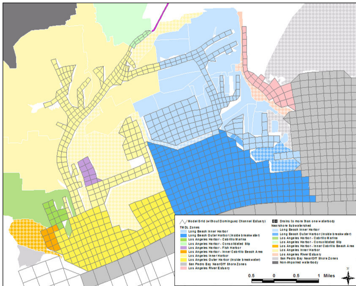
Figure 5-5. Nearshore subwatersheds (LSPC model) associated with TMDL (EFDC) model zones
